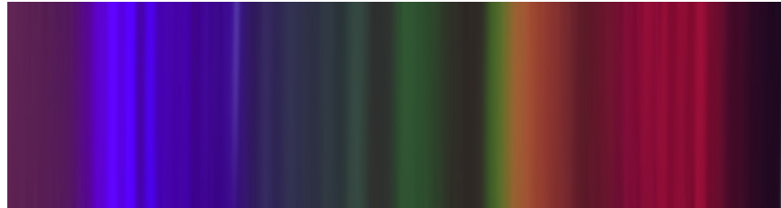
b / Visible spectrum of N_2 . Violet is on the left, red on the right.
